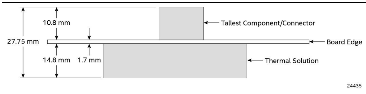
Figure 7. Board Height Dimensions
