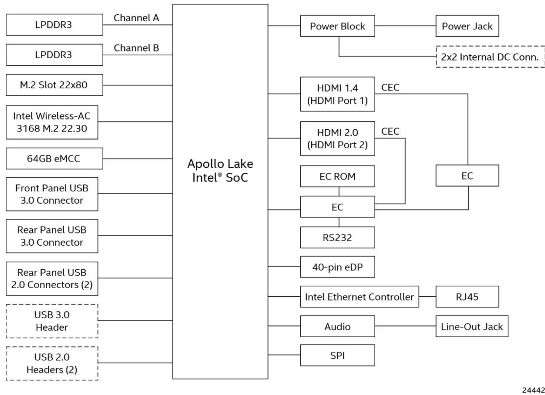
Figure 10. Block Diagram
