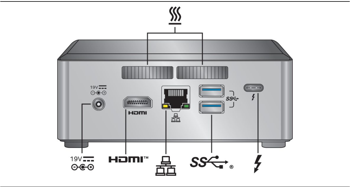
Figure 24. Intel NUC Kit NUC7i5BNH/NUC7i7BNH Features – Rear
