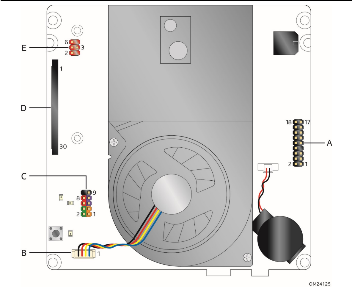
Figure 13. Connectors and Headers (Top)
