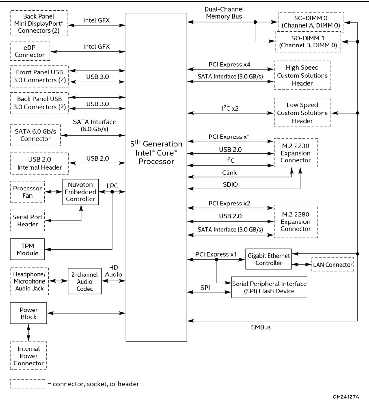
Figure 3. Block Diagram
