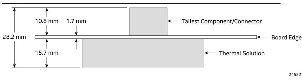
Figure 10. Board Height Dimensions
