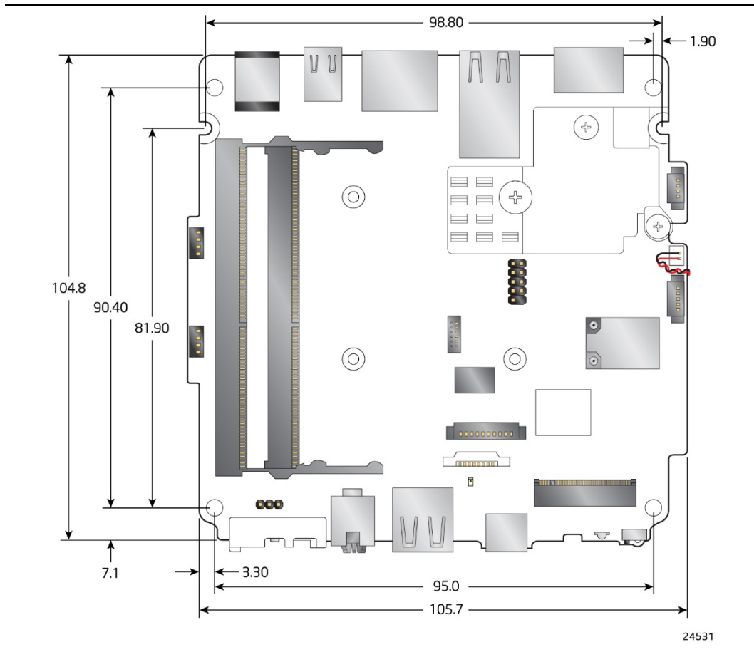
Figure 9. Board Dimensions
