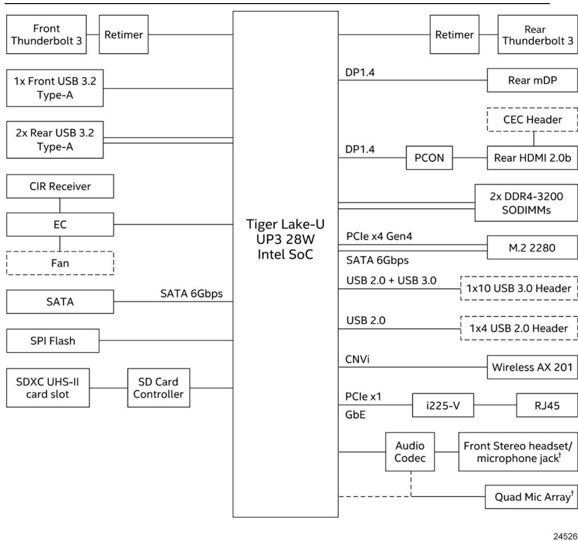
Figure 5. Block Diagram
