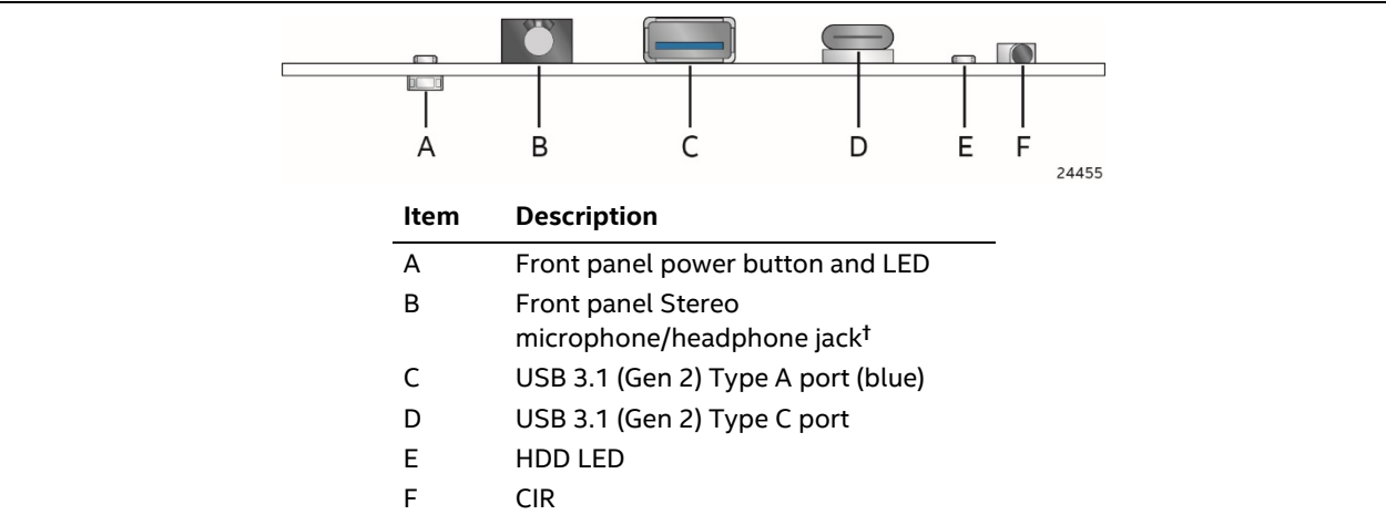
Figure 9. Front Panel Connectors
