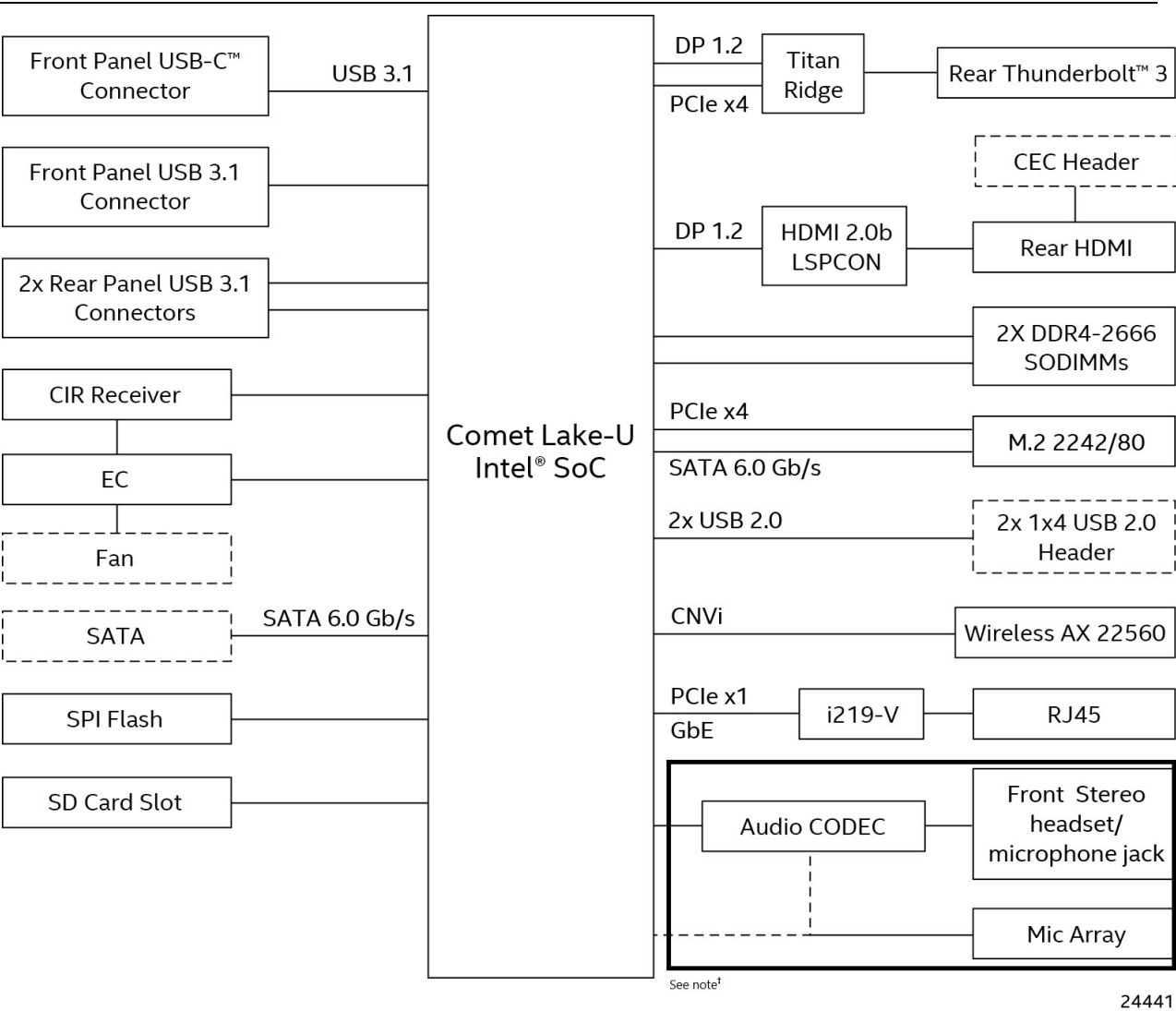
Figure 3. Block Diagram
