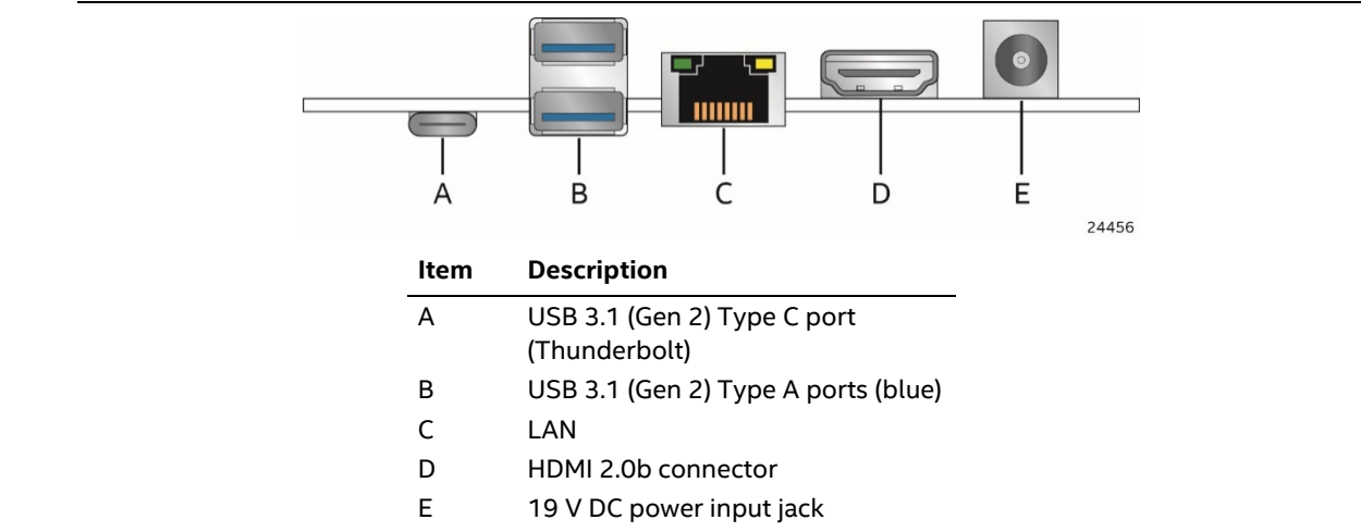
Figure 10. Back Panel Connectors
