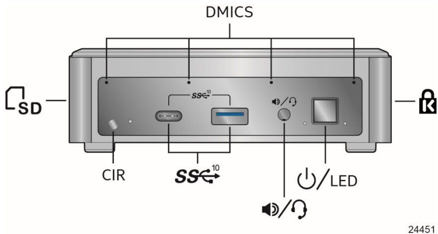
Figure 23. Intel NUC Kit NUC10i3FNK/NUC10i5FNK/NUC10i7FNK Features – Front
