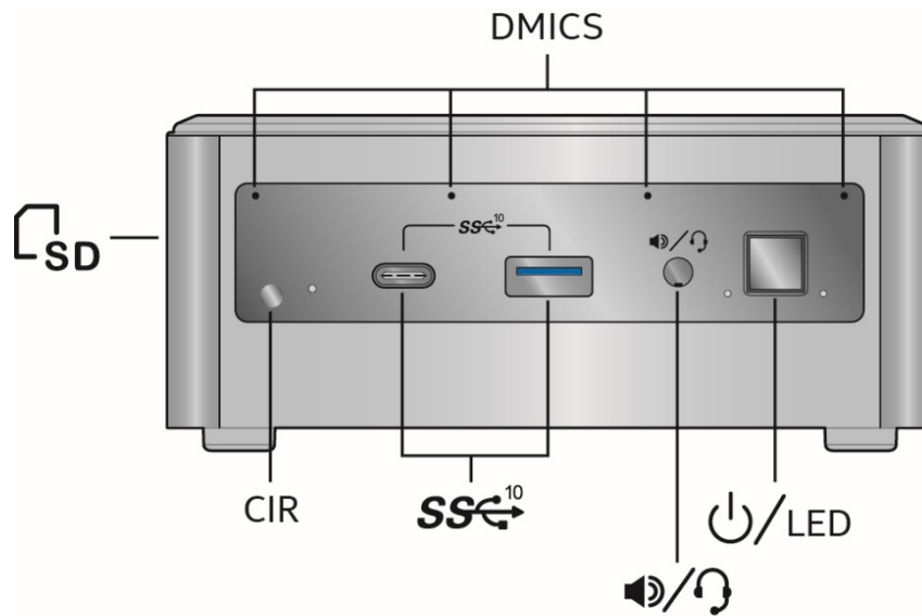
Figure 22. Intel NUC Kit NUC10i3FNH/NUC10i5FNH/NUC10i7FNH Features – Front
