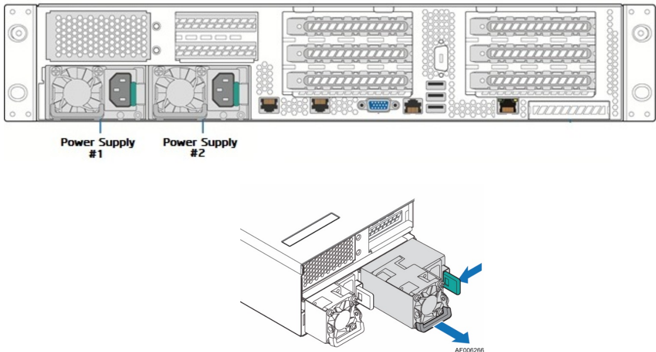
Figure 25. Power Supply Module Identification
