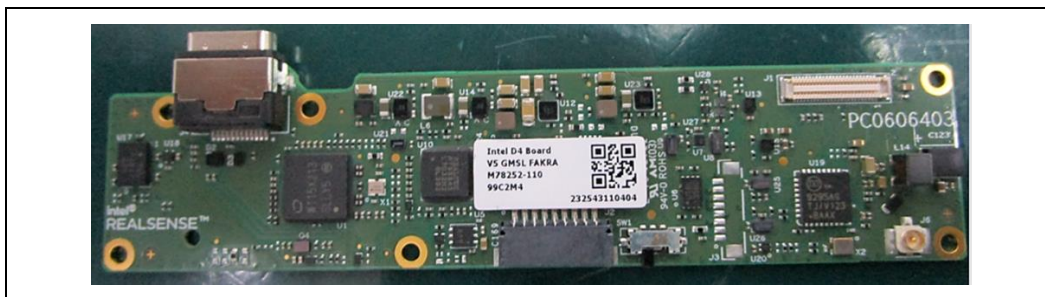
Figure 7-2. Intel® RealSense™ Vision Processor D4 Board V5
