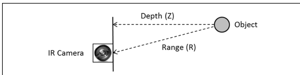
Figure 2-2. Depth Measurement (Z) versus Range (R)
