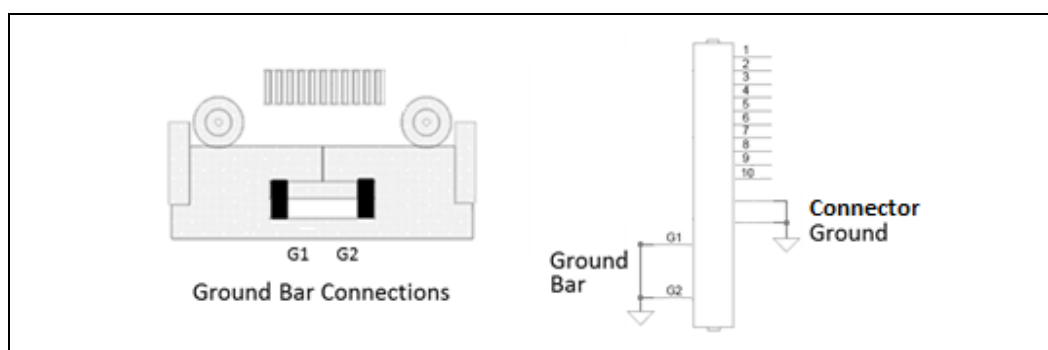
Figure 7-6. Receptacle Ground Bar Motherboard Connections
