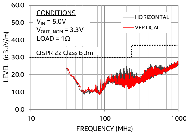
EMI Performance
