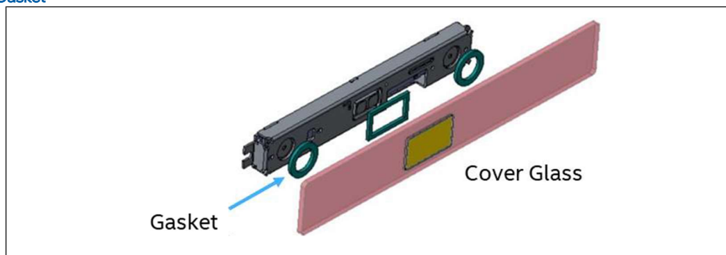
Figure 3-3: Gasket
