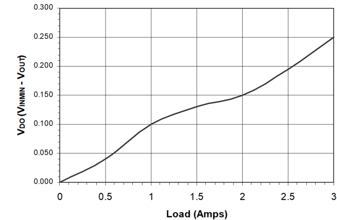
Drop-Out Voltage
