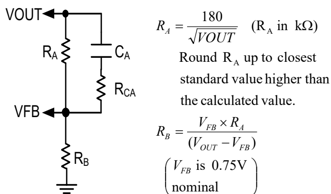
Figure 11. External Feedback Compensation. See Table 6 for details
