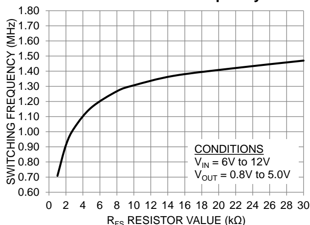
Figure 9. R FS versus Switching Frequency
