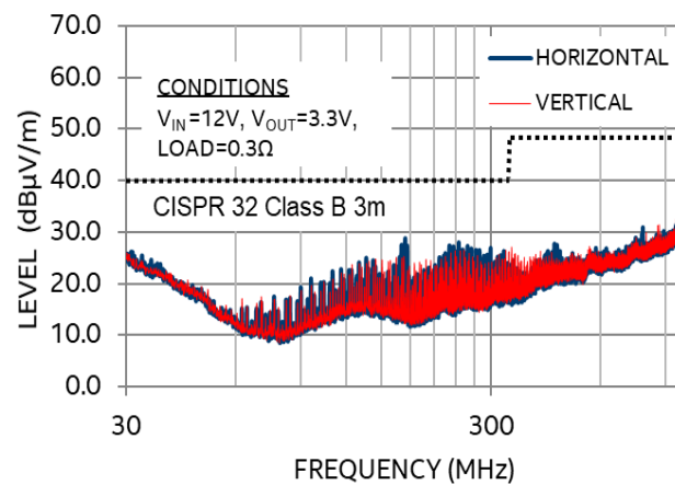
EMI Performance
