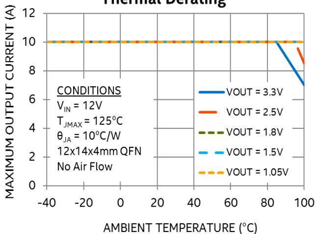
Thermal Derating
