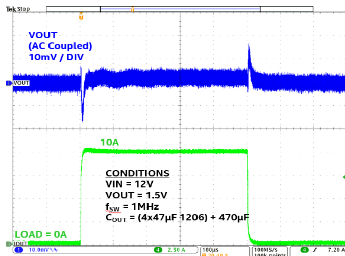
Load Transient 0 to 10A
