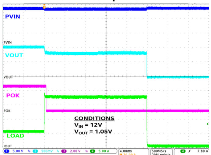
Short-circuit protection
