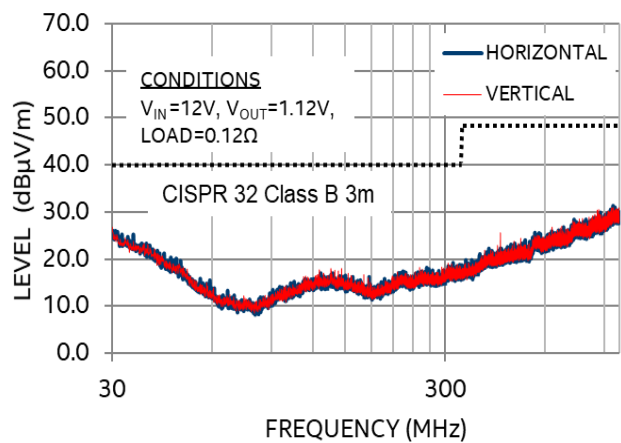
EMI Performance
