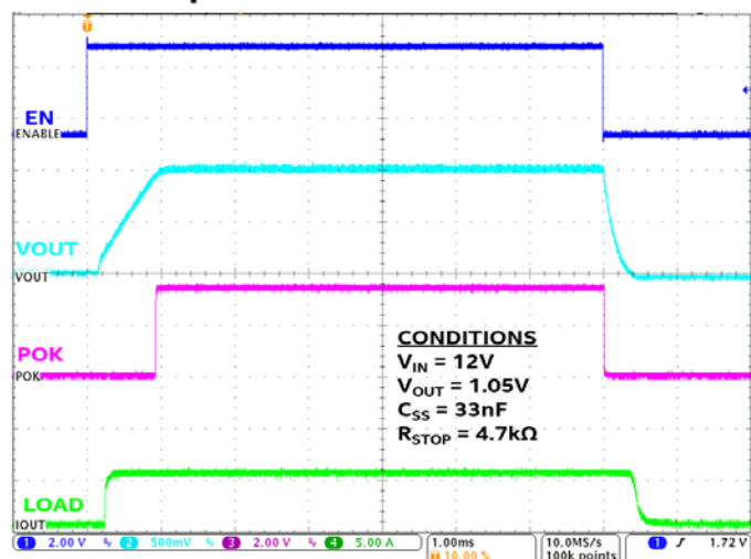
Startup and Shutdown at 5A Load
