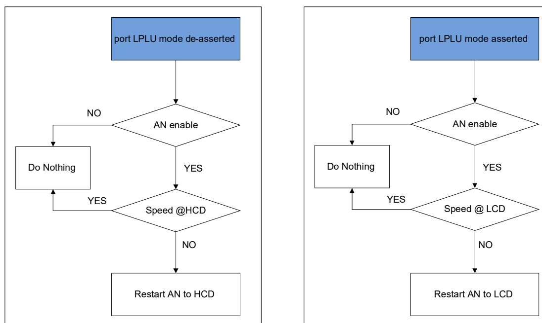
Figure 5-3. Link Speed Change on LPLU Assert/Clear
