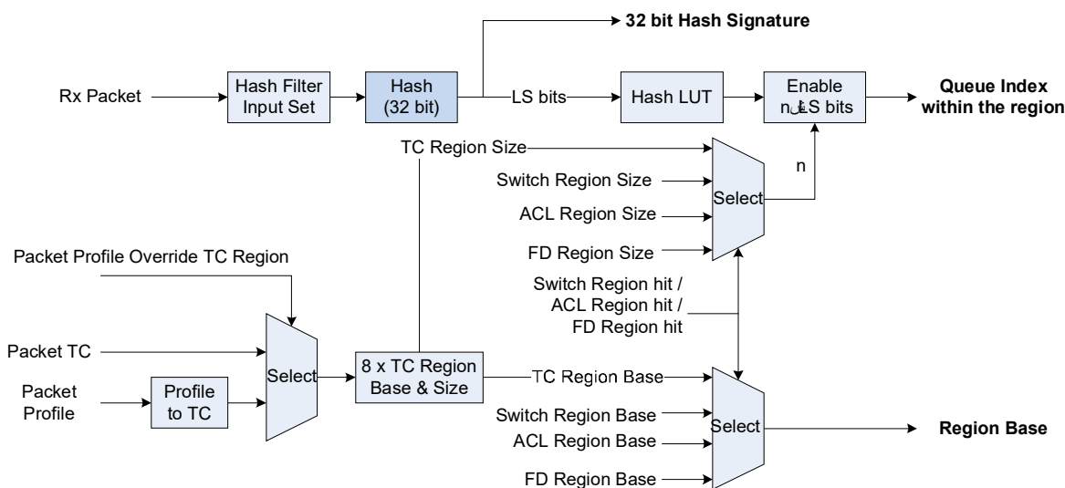
Figure 7-32. Hash Filter Block Diagram
