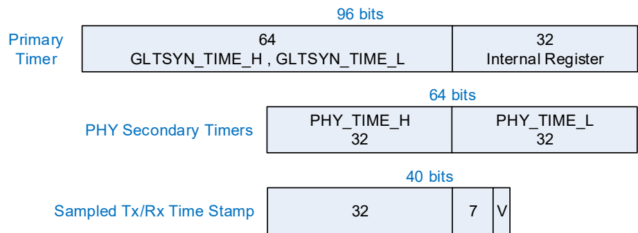
Figure 9-20. Sampled Timestamp
