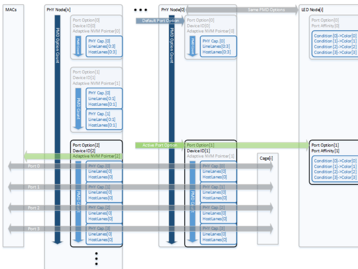
Figure 3-23. Port Options
