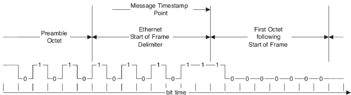
Figure 9-19. Timestamp Point
