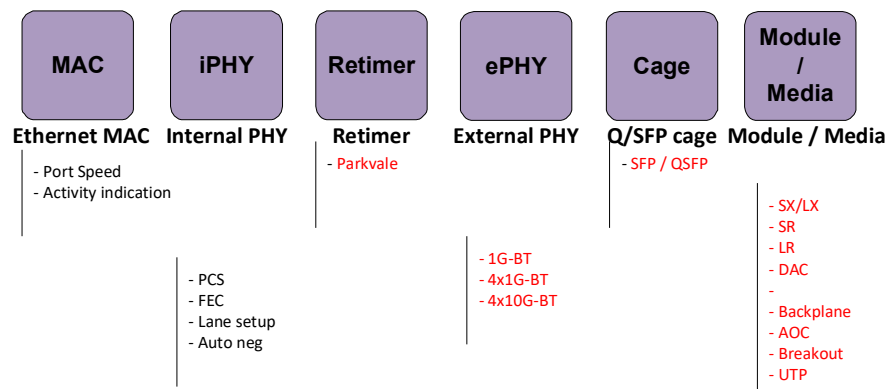
Figure 3-19. High-Speed PHY Chain
