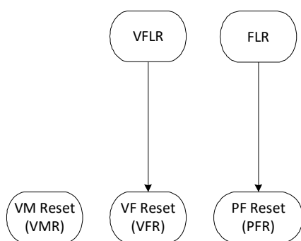
Figure 4-2. Function Virtual Resets
