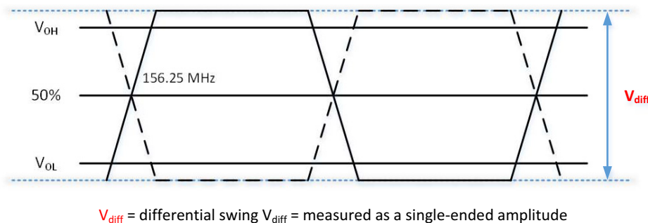
Figure 16-9. Differential Swing V_{diff}
