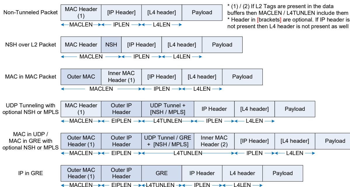
Figure 10-11. Transmit L3 and L4 Header Lengths (in Host Memory) for Integrity Offload
