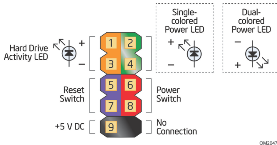
Figure 13. Connection Diagram for Front Panel Header (2.0 mm Pitch)
