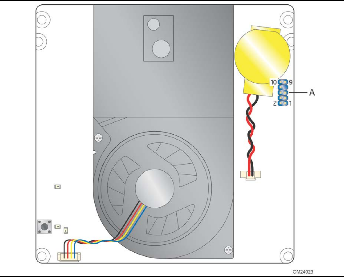
Figure 11. Header (Top)
