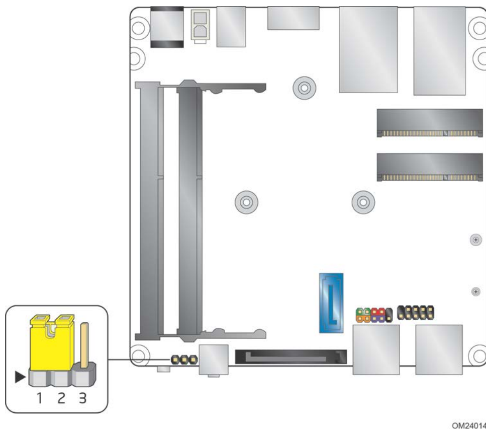
Figure 16. Location of the BIOS Security Jumper
