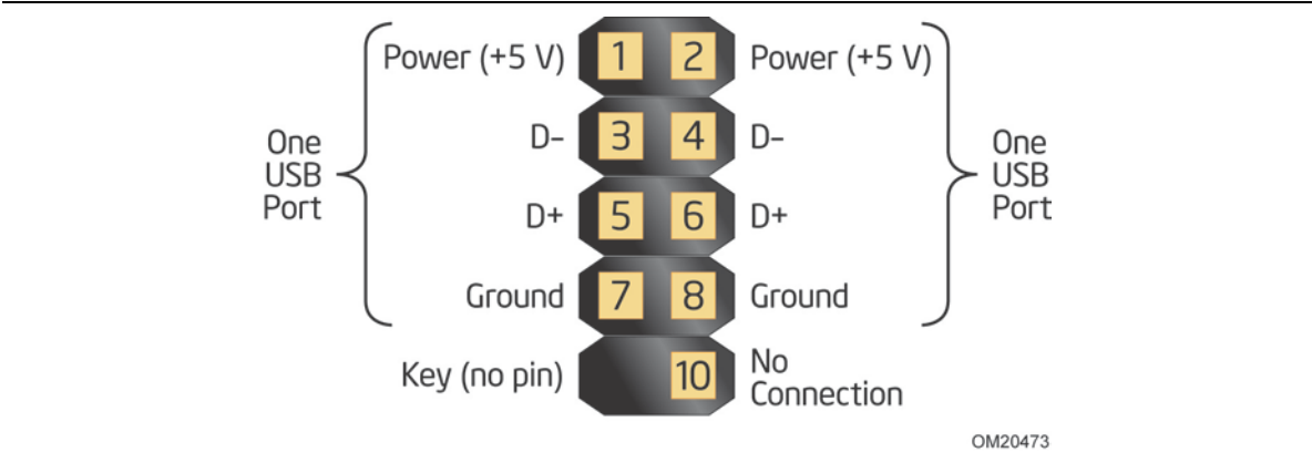
Figure 14. Connection Diagram for Internal USB 2.0 Dual-Port Header (2.0 mm Pitch)
