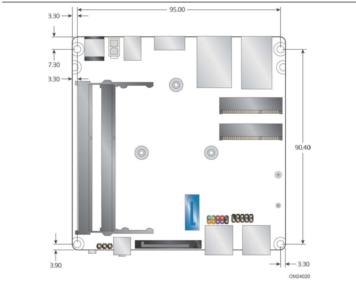
Figure 17. Board Dimensions
