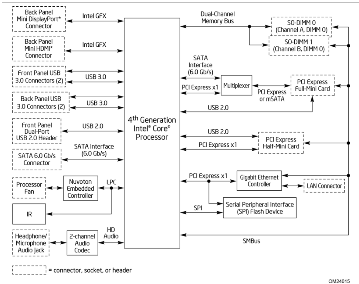
Figure 3. Block Diagram
