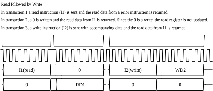
Figure 5-13: HPS SPI Read Timing (Read/Write)
