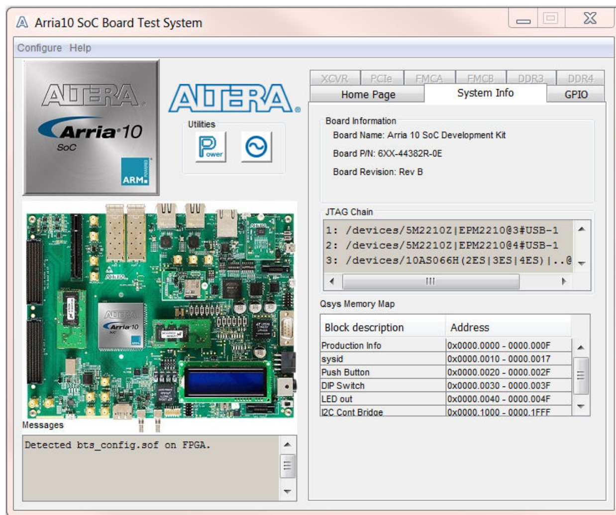
Figure 4-4: The System Info Tab
