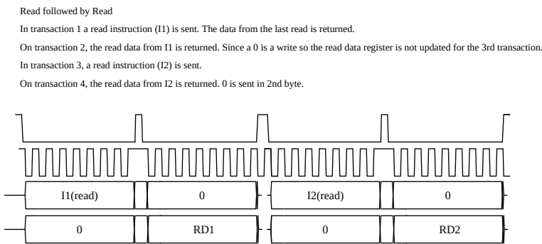
Figure 5-14: HPS SPI Read Timing (Read/Read)
