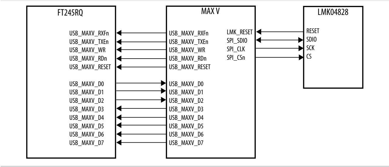
Figure 5-9: LMK04828 Controller
