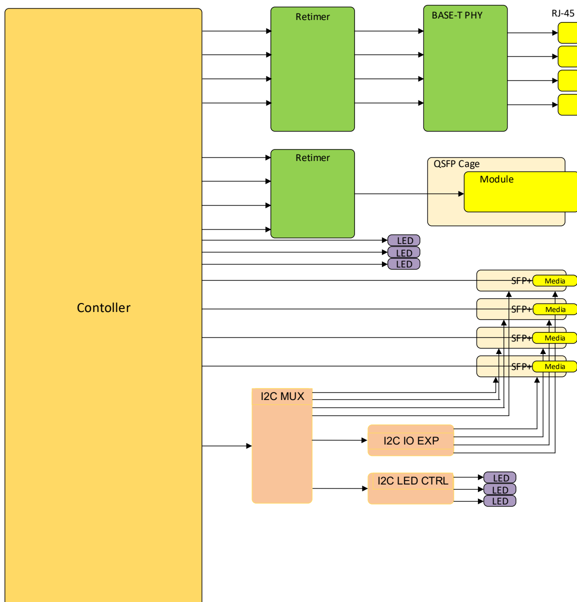
Figure 3-18. Topology Schematic
