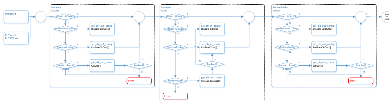
Figure 3-15. SyncE Initialization
