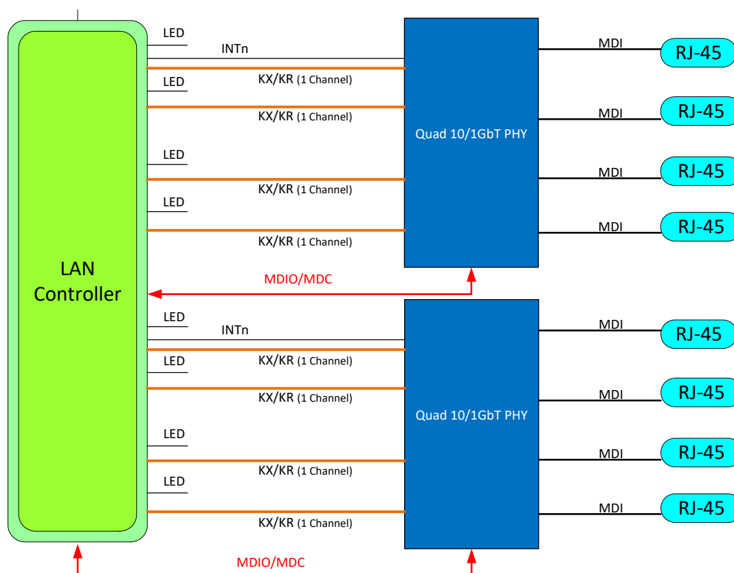
Figure 3-14. Octal 10GBASE-T/1GBASE-T
