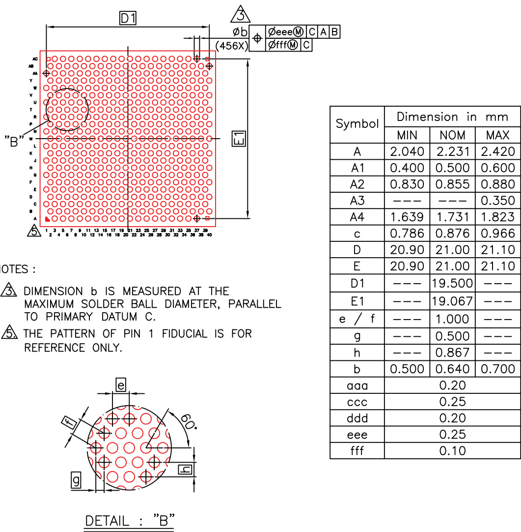
Figure 16-15. E810-XXVAM2 Mechanical Package Diagram (Bottom View)
