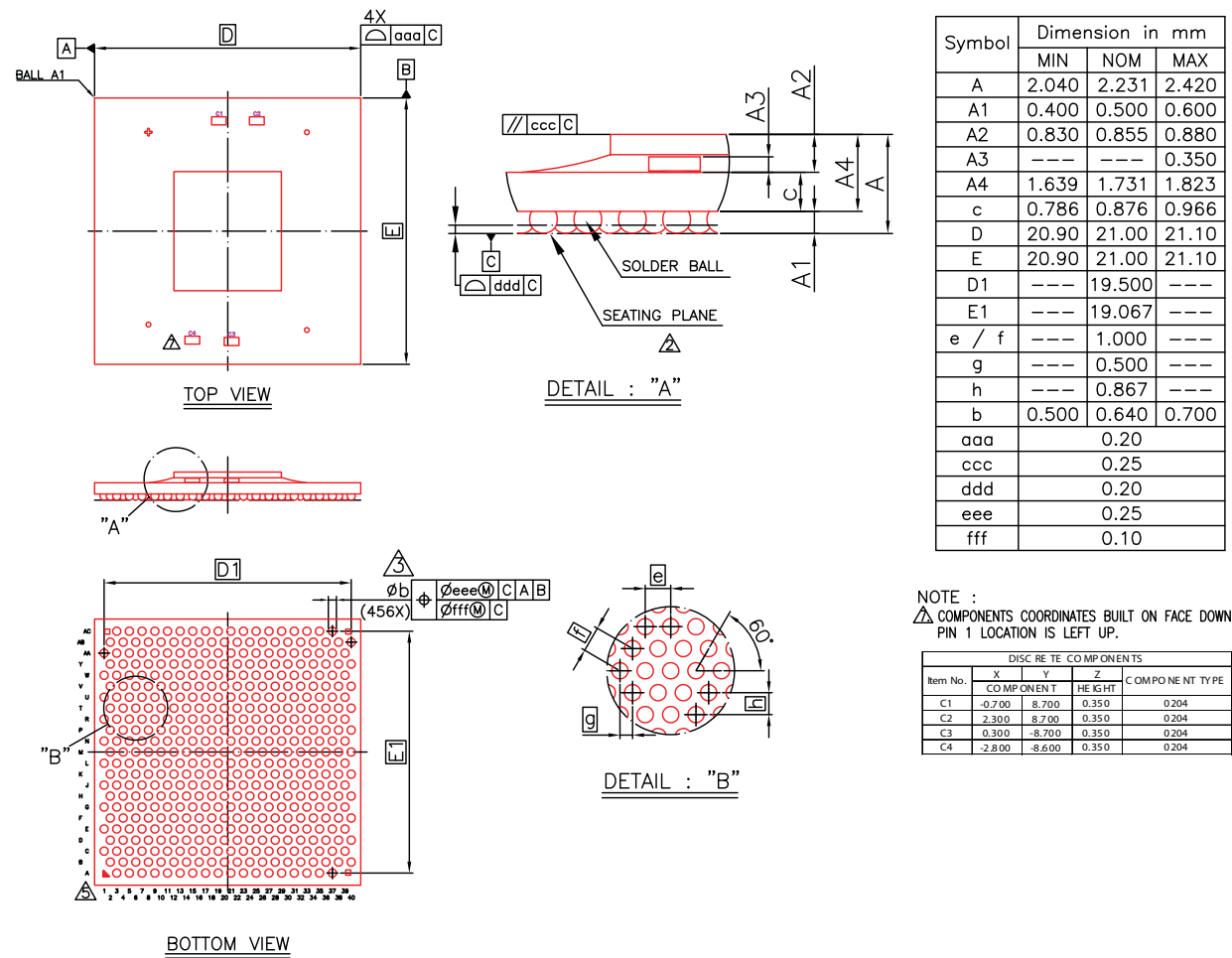
Figure 18-2. E810-XXVAM2 FCBGA Mechanical Illustration
