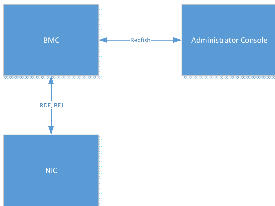
Figure 12-16. RDE Setup
