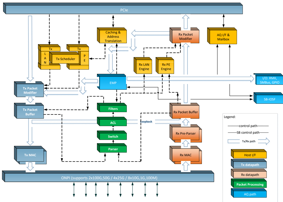
Figure 8-2. E810 Block Diagram
