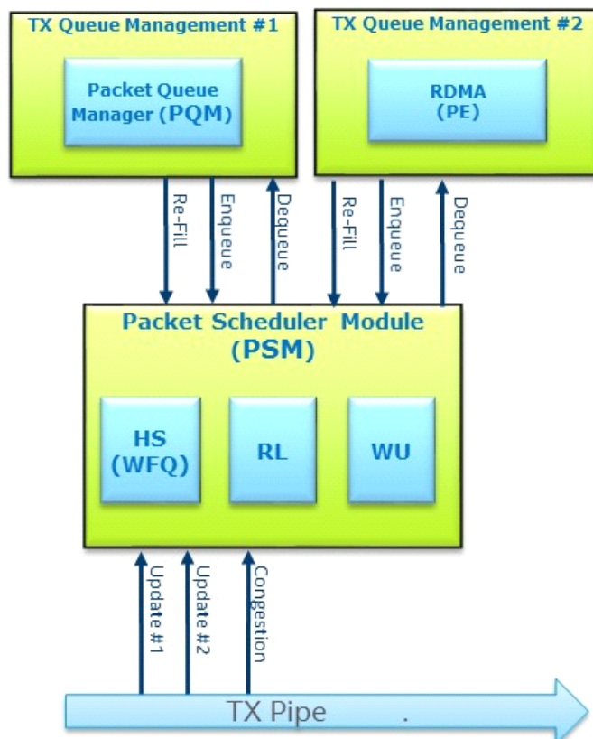
Figure 8-28. Parallel RDMA-PQM Connectivity to PSM
