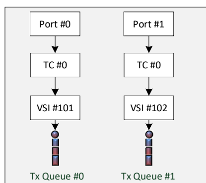
Figure 8-27. Example of Initial Configuration of a Dual Port Device
