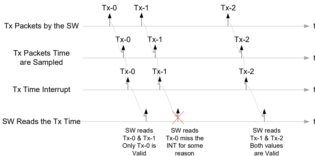
Figure 9-21. Sampled Timestamp
