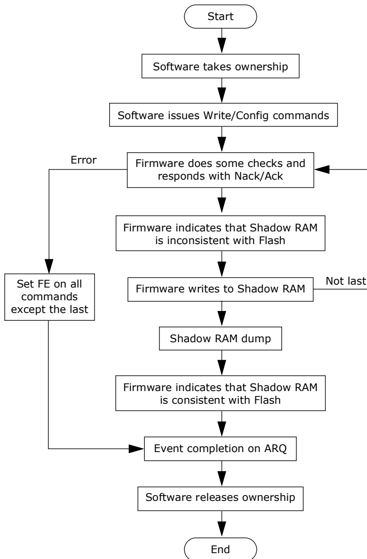
Figure 3-29. PFA Update Flow
