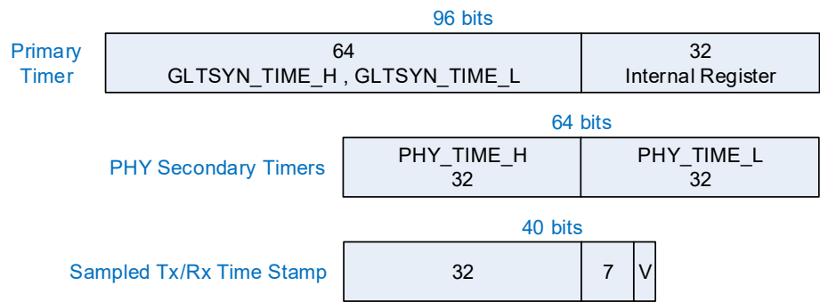
Figure 9-20. Sampled Timestamp
