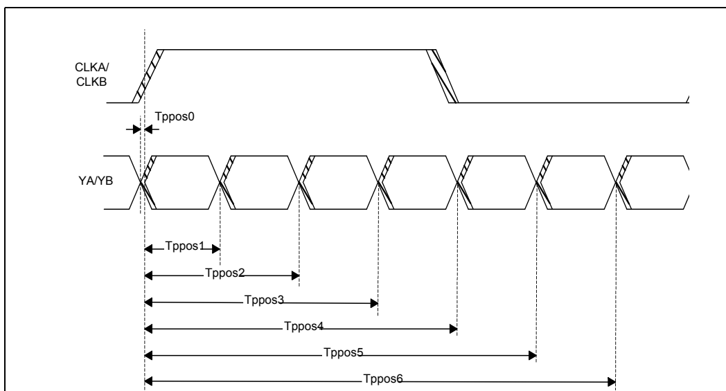
Figure 8-9. Clock Timing
