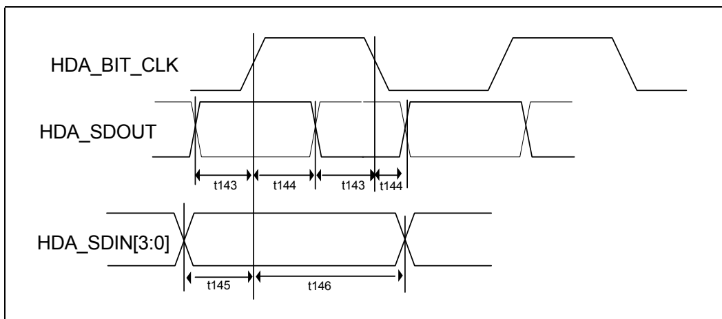
Figure 8-21. Intel® High Definition Audio Input and Output Timings
