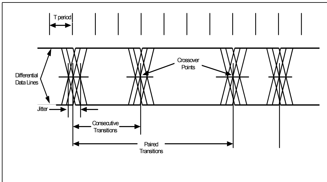
Figure 8-16. USB Jitter
