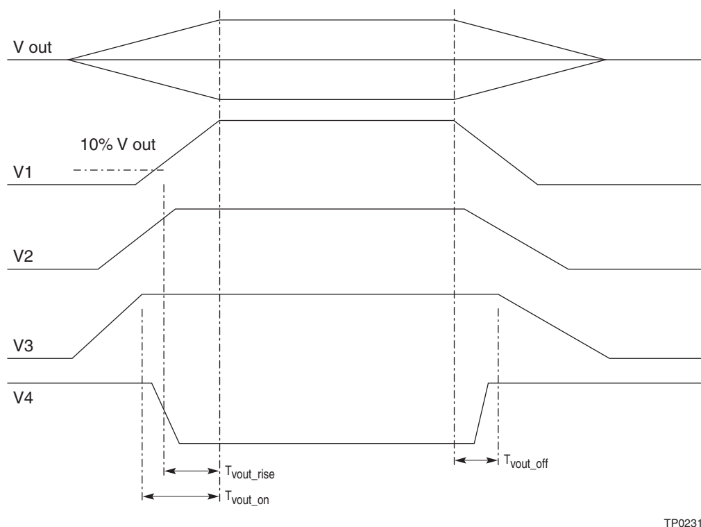
Figure 25. Output Voltage Timing
