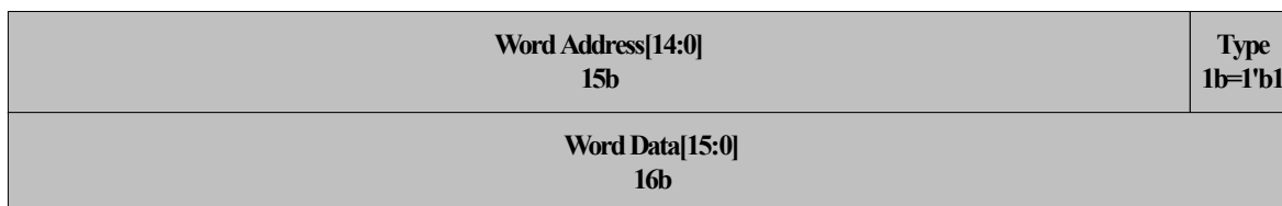
Figure 6-2. Shadow RAM Word Write Command
