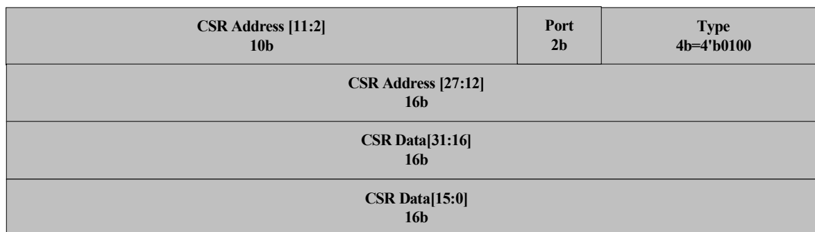
Figure 6-3. CSR Write Command (with Port Number)
