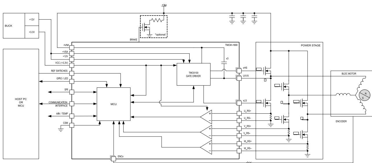
Figure 14: Bottom Shunt Current Sense
