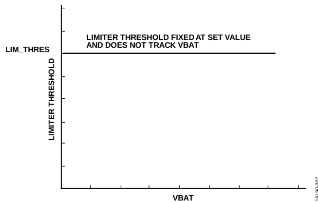
Figure 75. Limiter Fixed (LIM_EN = 0b11, VBAT_TRACK = 0b0)
