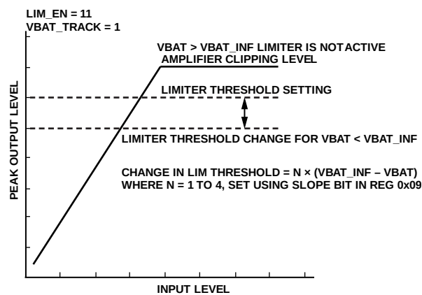
Figure 76. Limiter Example (LIM_EN = 0b11, VBAT_TRACK = 0b1)
