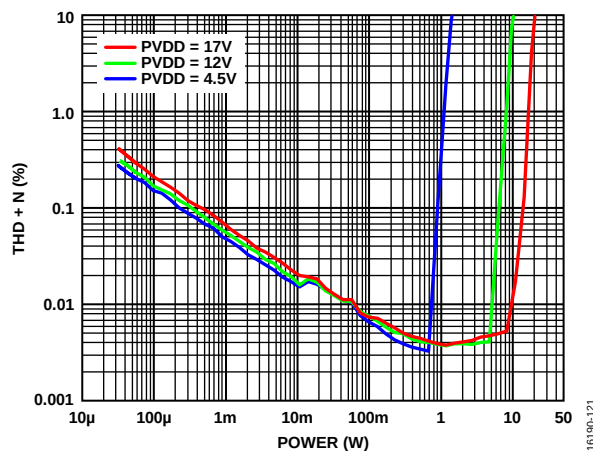
Figure 27. THD + N vs. Output Power, R_L = 8\ \Omega , Analog Gain = 16
