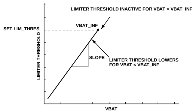
Figure 77. Output Level vs. VBAT in Limiter Tracking Mode (LIM_EN = 0b11, VBAT_TRACK = 0b1)
