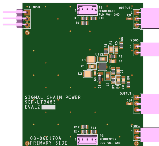
Figure 1. SCP-LT3463-EVALZ Board
