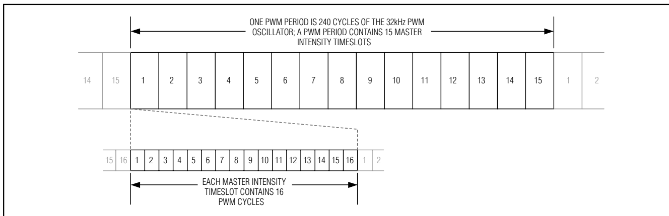
Figure 12. PWM Timing
