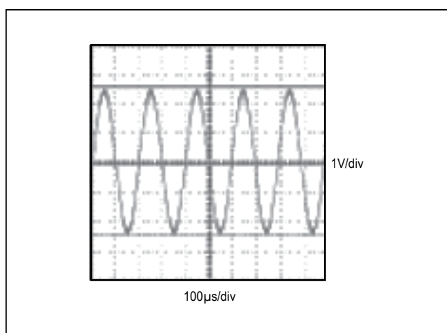
Figure 1. Rail-to-Rail Output Operation
