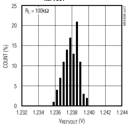
V_{REFVOUT} DISTRIBUTION
