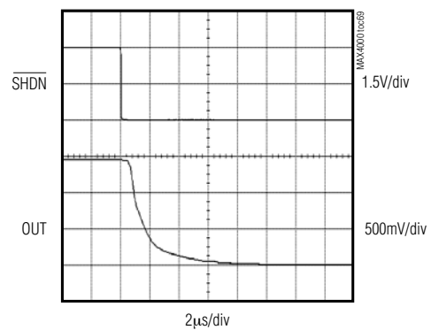
\overline{SHDN} RESPONSE TIME
