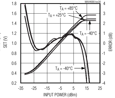
MAX4002 SET AND LOG CONFORMANCE vs. INPUT POWER AT 2.5GHz (μMAX)
