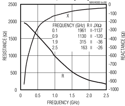
MAX4002 INPUT IMPEDANCE vs. FREQUENCY (UCSP)
