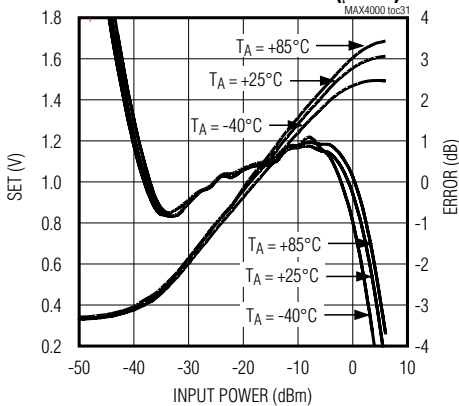
MAX4000 SET AND LOG CONFORMANCE vs. INPUT POWER AT 2.5GHz (UCSP)
