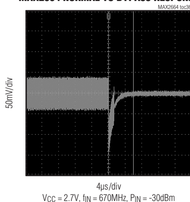
MAX2664 NORMAL TO BYPASS RESPONSE
