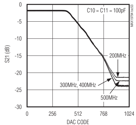
ATTENUATION vs. DAC CODE
