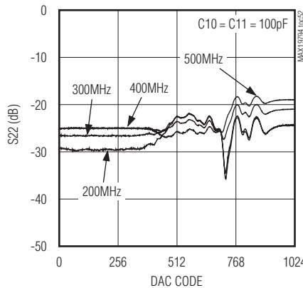
OUTPUT MATCH vs. DAC CODE
