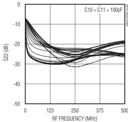
OUTPUT MATCH vs. RF FREQUENCY OVER CODE SETTINGS
