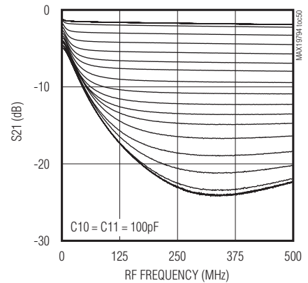
ATTENUATION vs. RF FREQUENCY OVER CODE SETTINGS
