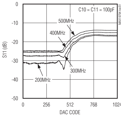
INPUT MATCH vs. DAC CODE
