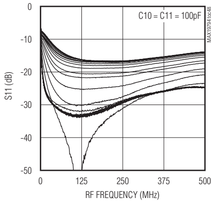
INPUT MATCH vs. RF FREQUENCY OVER CODE SETTINGS
