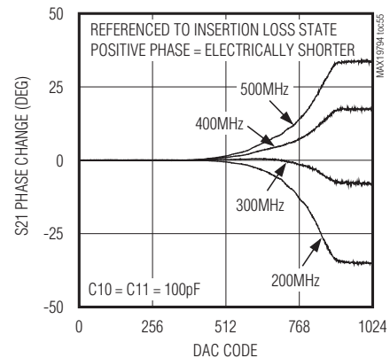
S21 PHASE CHANGE vs. DAC CODE
