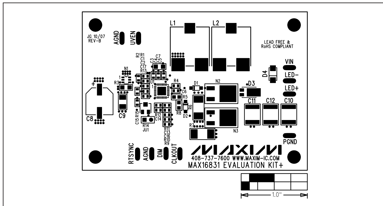
Figure 2. MAX16831 EV Kit Component Placement Guide—Components Side
