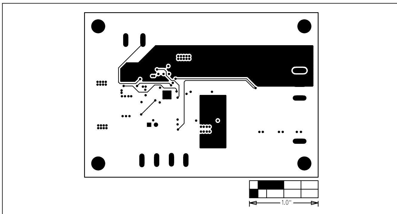
Figure 5. MAX16831 EV Kit PCB Layout—VCC Layer 3
