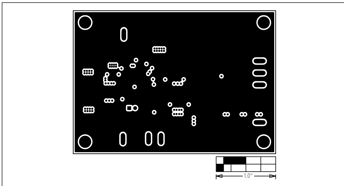
Figure 4. MAX16831 EV Kit PCB Layout—GND Layer 2
