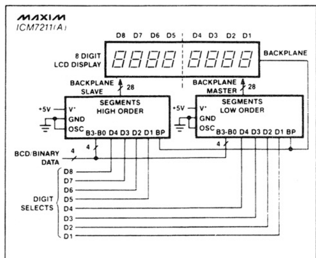
Figure 14. Two ICM7211's Driving 8-Digit LCD Display.
