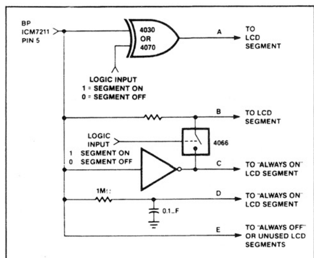
Figure 13. Driving Annunciators, Flags and Decimal Points.
