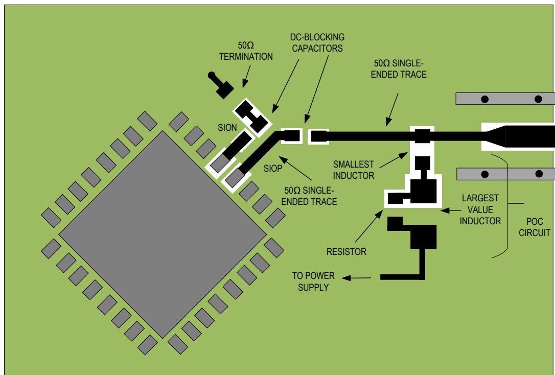
Figure 22. Coax PoC Layout Example
