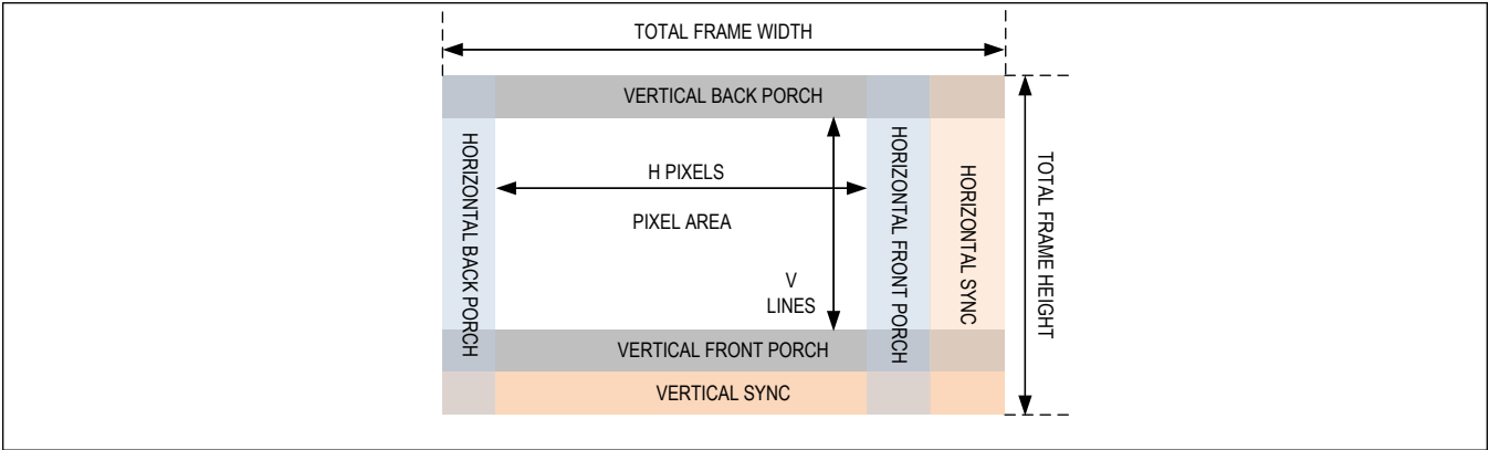
Figure 28. Video Timing
