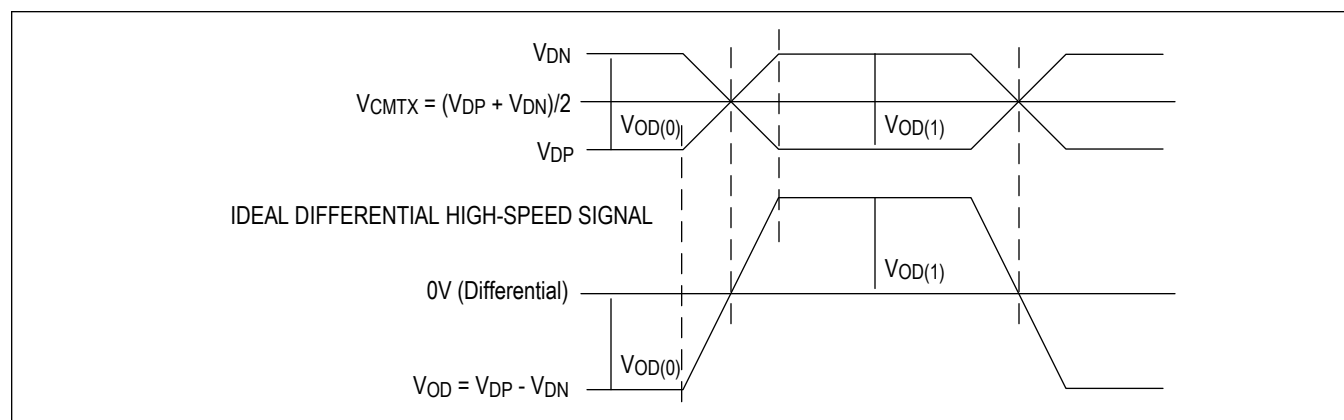
Figure 3. D-PHY Ideal Single-Ended and Resulting Differential HS Signals
