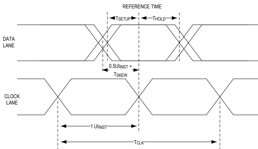
Figure 11. D-PHY Data Clock Timing
