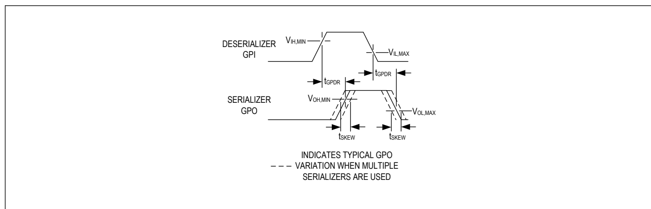
Figure 16. GMSL2 GPI-to-GPO Delay and Skew
