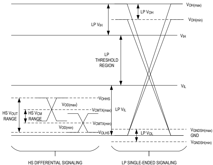
Figure 10. D-PHY Signaling Levels
