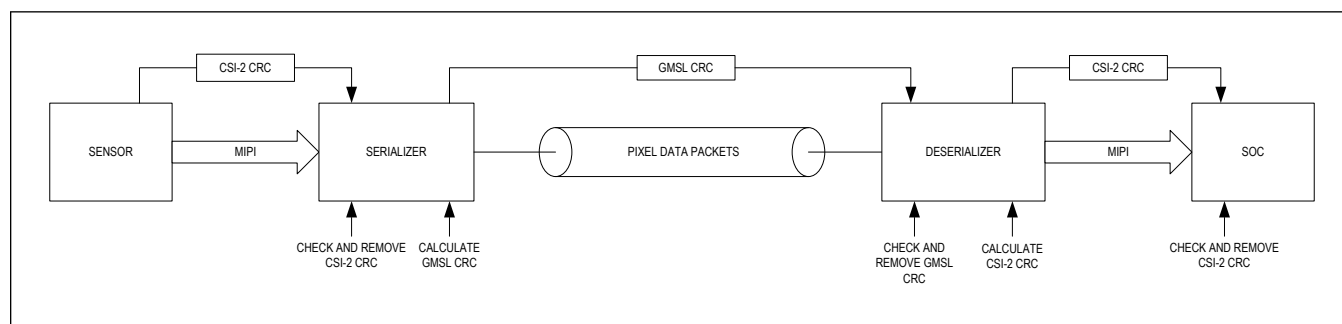
Figure 21. Pixel Mode
