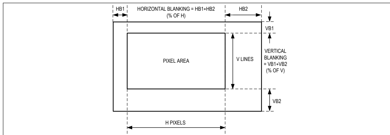
Figure 19. Video Frame Format for Bandwidth Calculation
