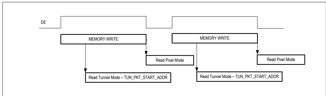
Figure 23. GMSL2 Memory Reading and Writing
