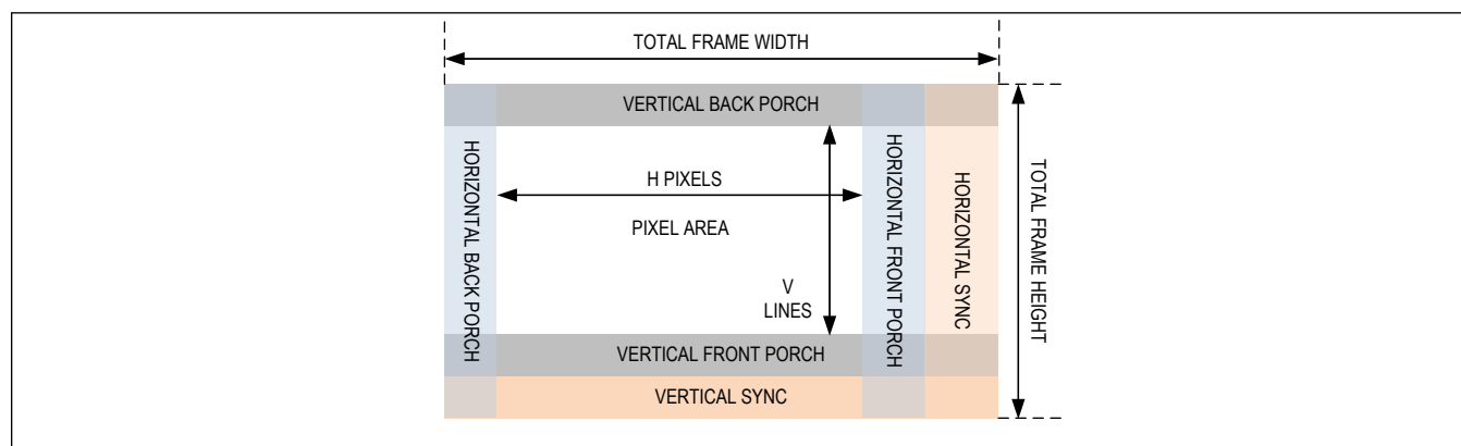
Figure 34. Video Timing
