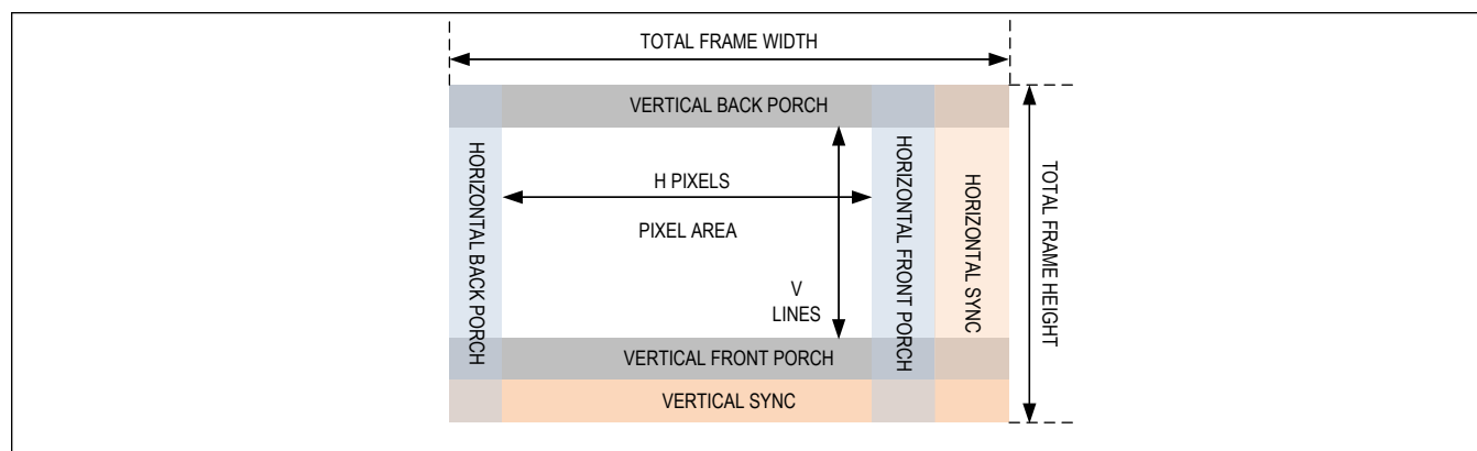
Figure 20. Video Timing
