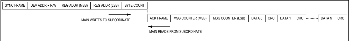
Figure 32. UART Multiple-Byte Read Transaction with CRC (message counter enabled)
