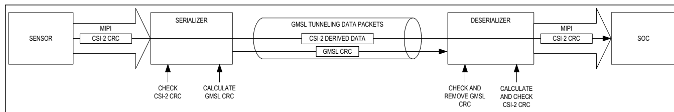
Figure 22. Tunnel Mode
