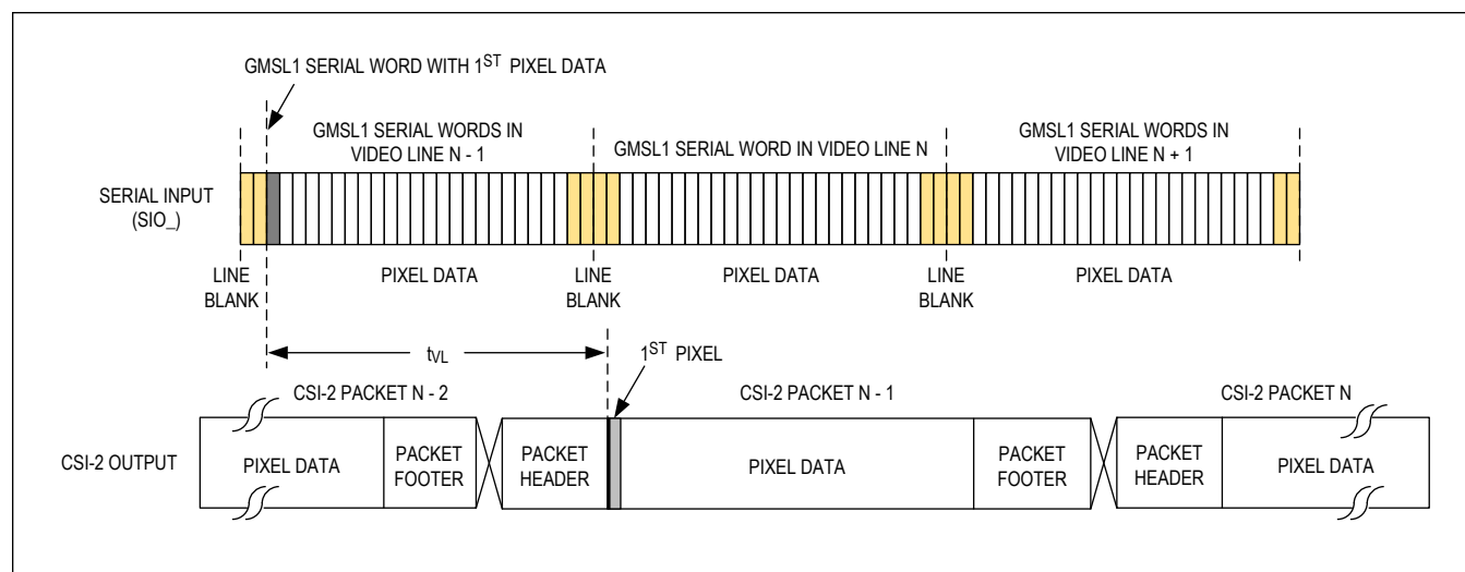
Figure 8. GMSL1 Video Latency
