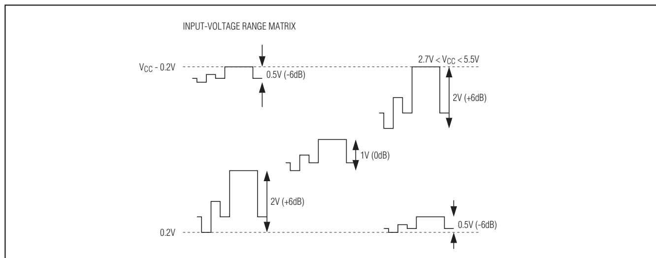
Figure 3. Input-Voltage Range Matrix
