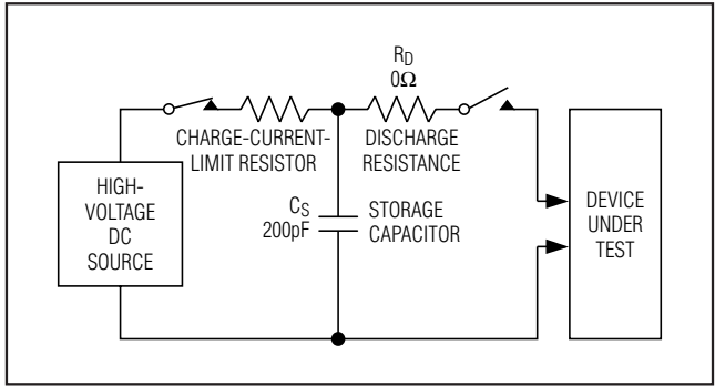
Figure 16. Machine Model ESD Test Circuit.
