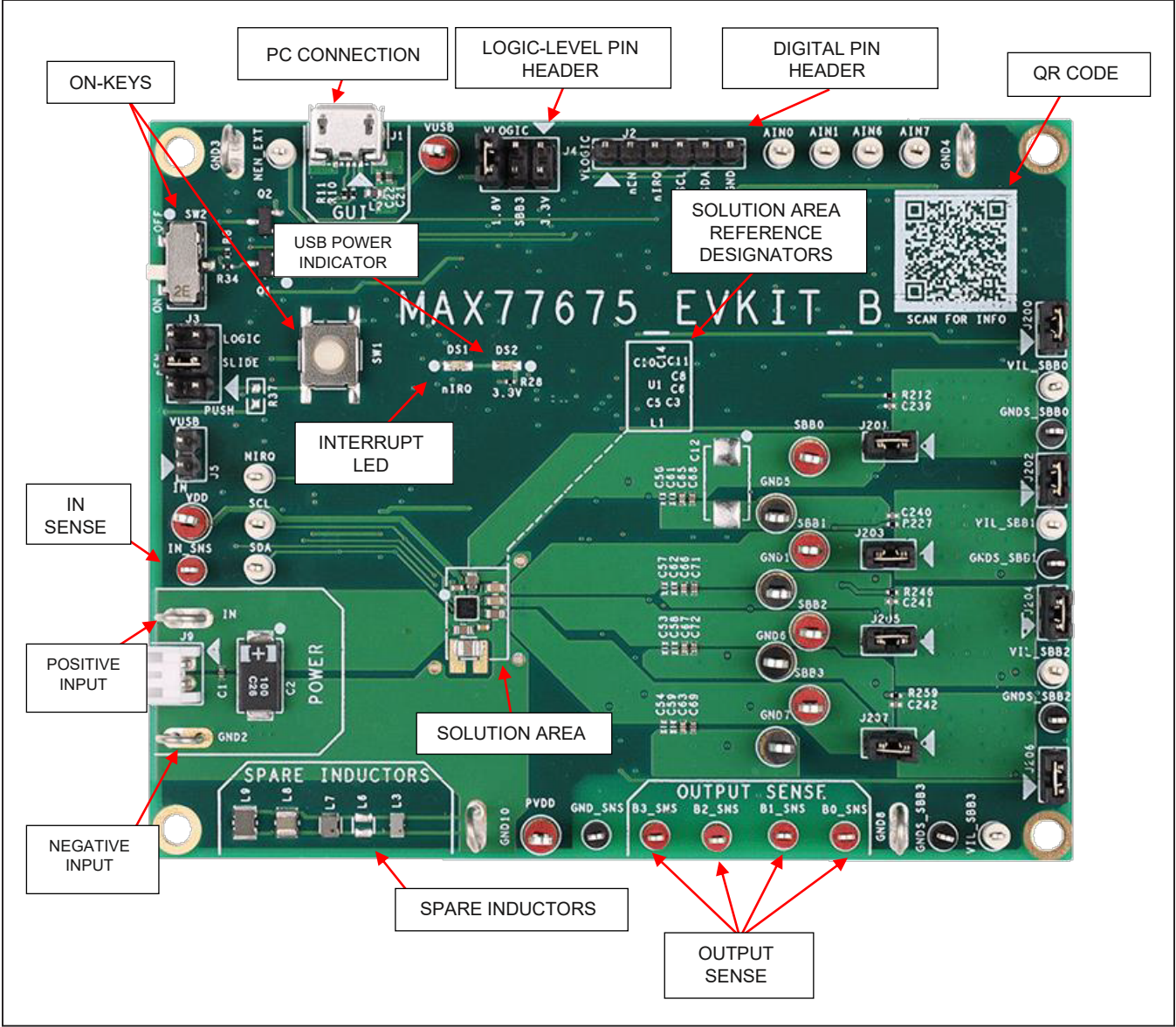
Figure 3. MAX77675 EV Kit Top View
