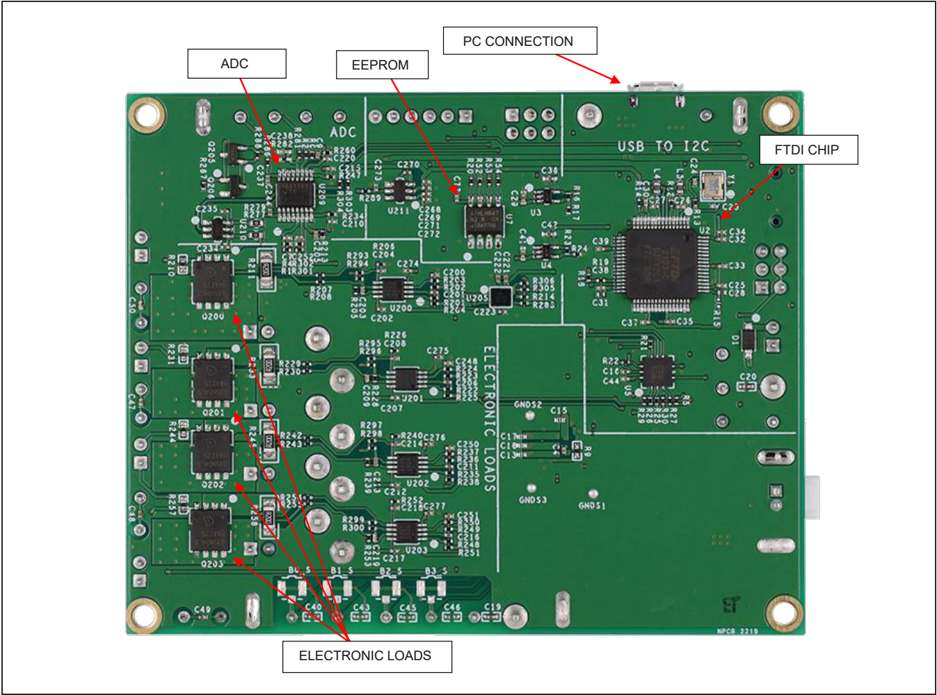
Figure 4. MAX77675 EV Kit Bottom View
