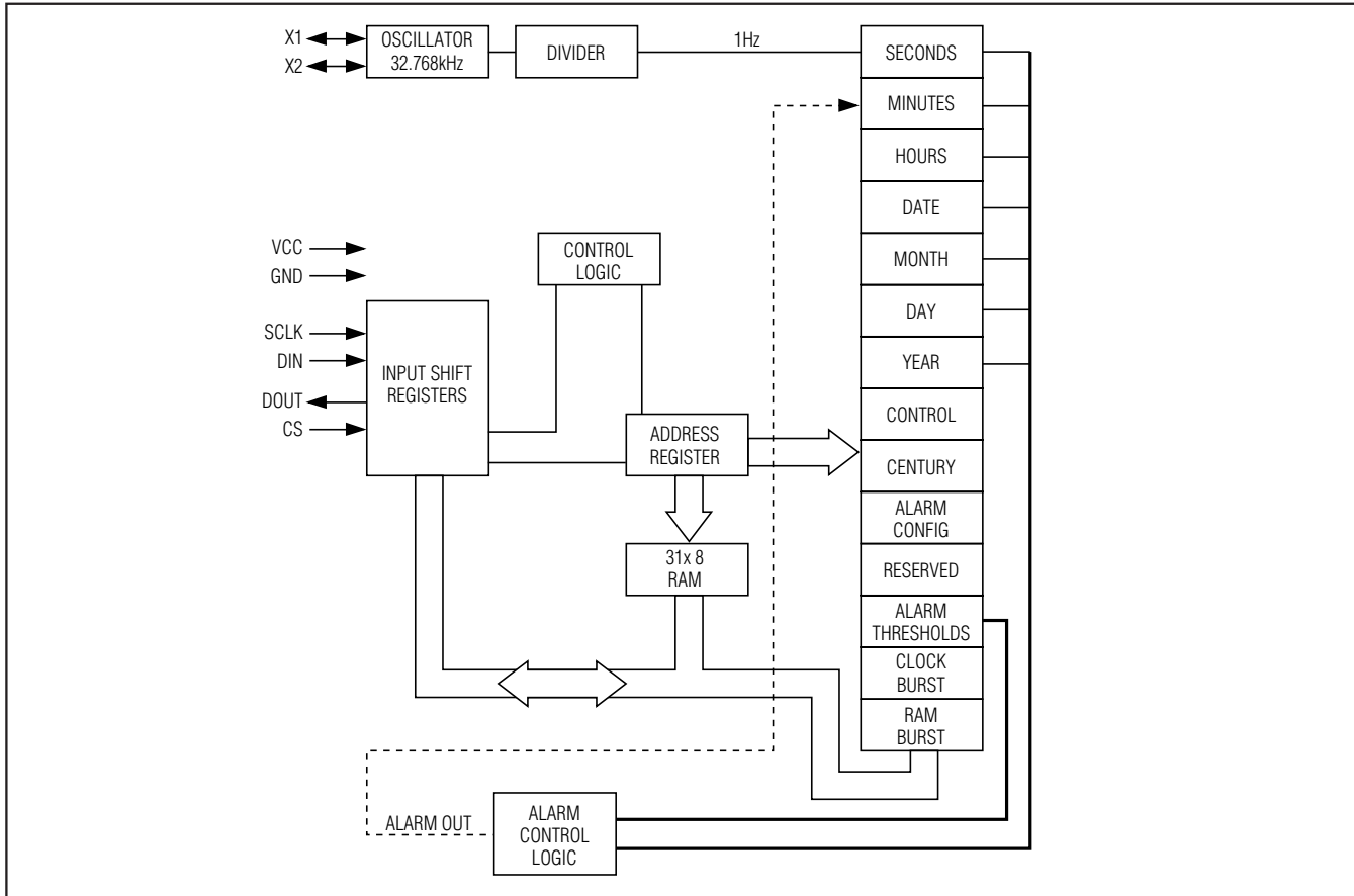
Functional Diagram
