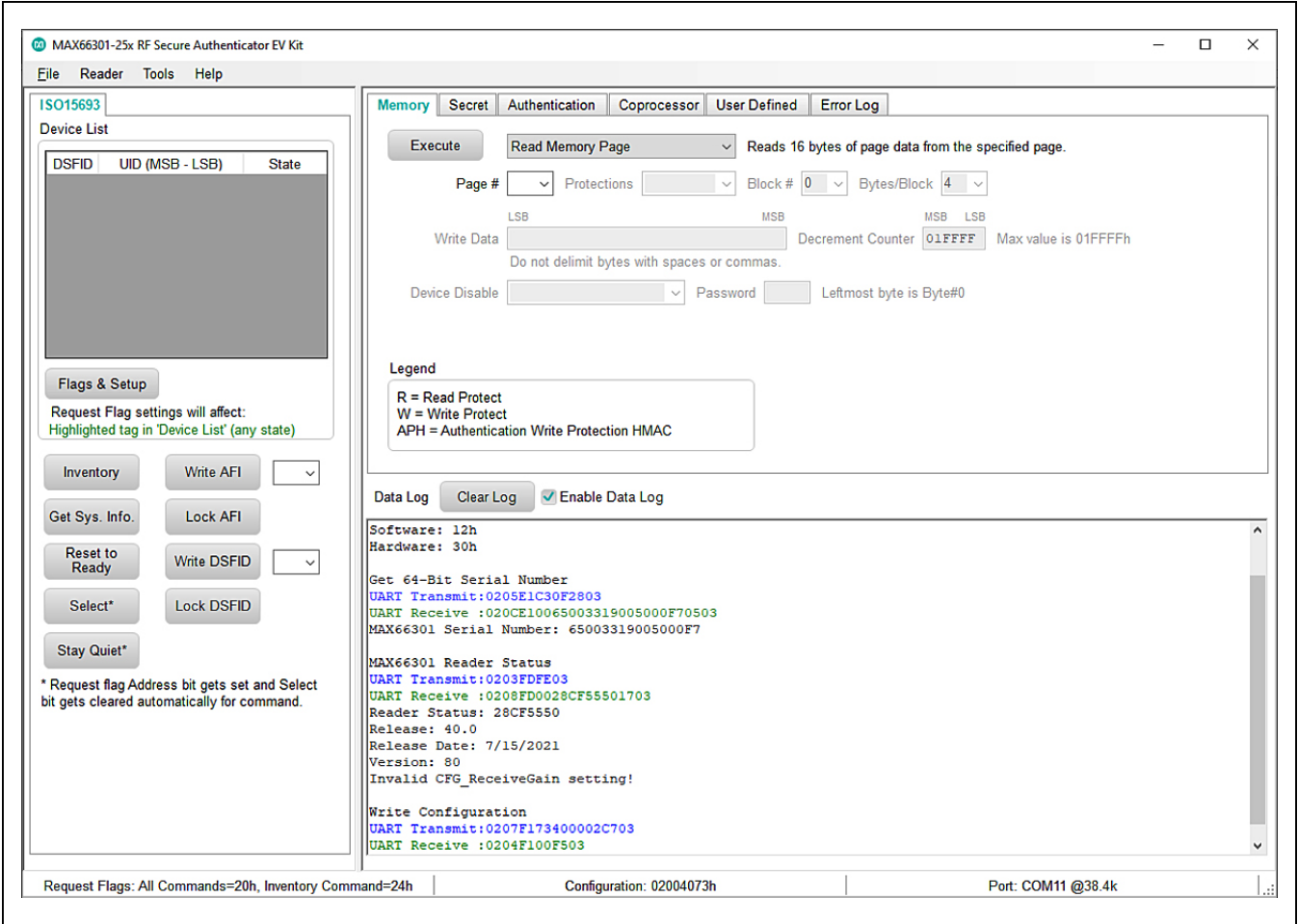
Figure 4. MAX66301-25x EV Kit GUI
