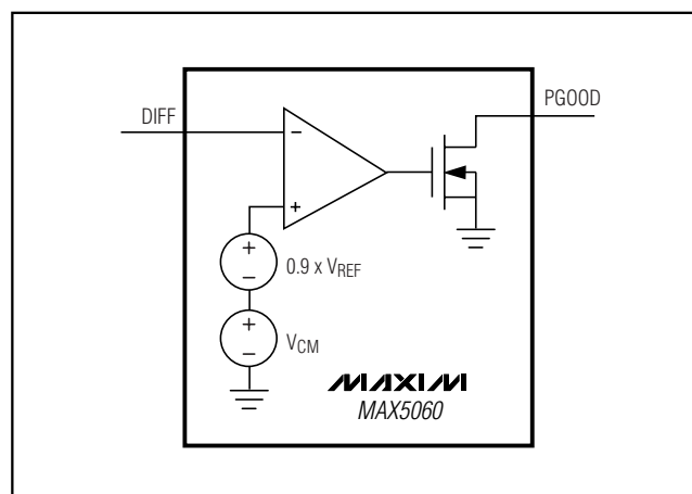
Figure 8. PGOOD Generator
