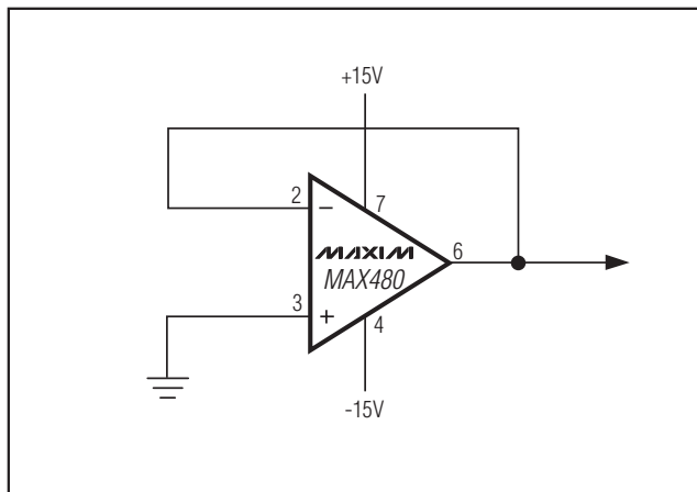
Figure 2. Burn-In Circuit
