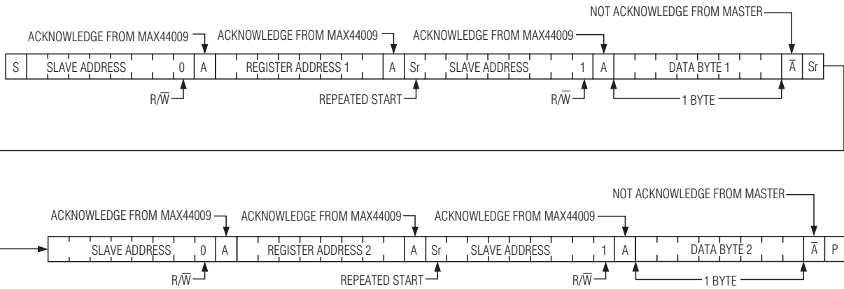
Figure 8. Reading Two Registers Consecutively Without a STOP Condition in Between Reads
