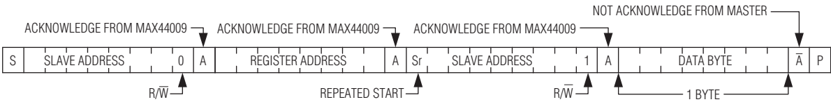
Figure 7. Reading 1 Indexed Byte of Data from the IC
