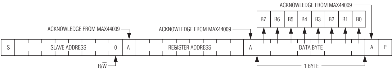
Figure 6. Writing 1 Byte of Data to the IC
