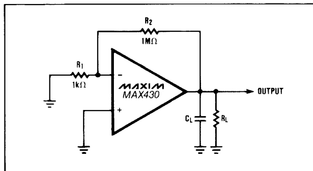
Figure 1. Test Circuit
