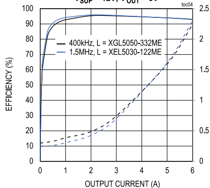
EFFICIENCY AND POWER LOSS vs. OUTPUT CURRENT FPWM MODE V_{SUP} = 12V , V_{OUT} = 5V
