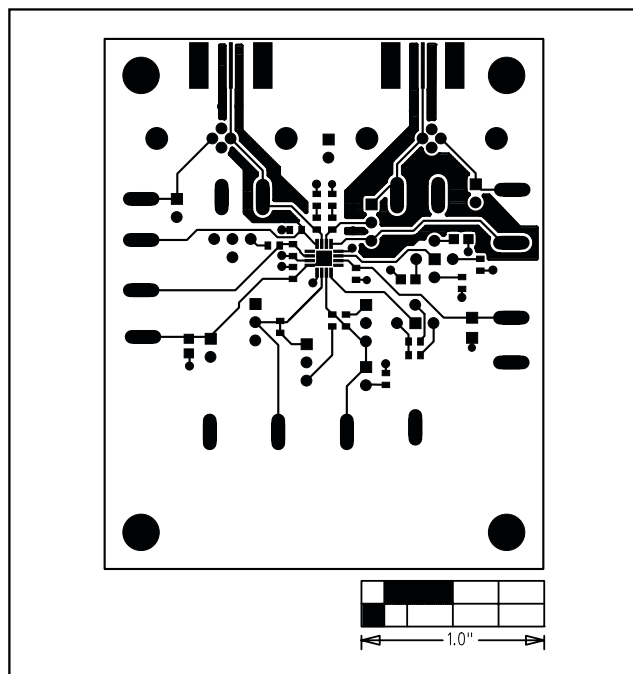
Figure 3. MAX4206 EV Kit PC Board Layout—Component Side
