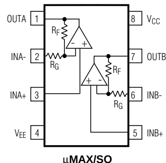
MAXIM MAX4274
