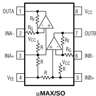
MAXIM MAX4275
