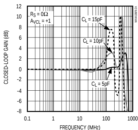
Figure 2a. MAX4108 Response vs. Capacitive Load—No Resistive ( R_S ) Isolation (circuit shown in Figure 1a)
