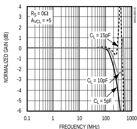
Figure 2c. MAX4308 Response vs. Capacitive Load—No Resistive ( R_S ) Isolation (circuit shown in Figure 1a)
