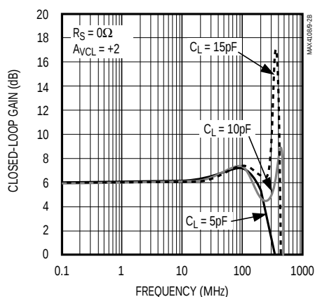
Figure 2b. MAX4109 Response vs. Capacitive Load—No Resistive ( R_S ) Isolation (circuit shown in Figure 1a)
