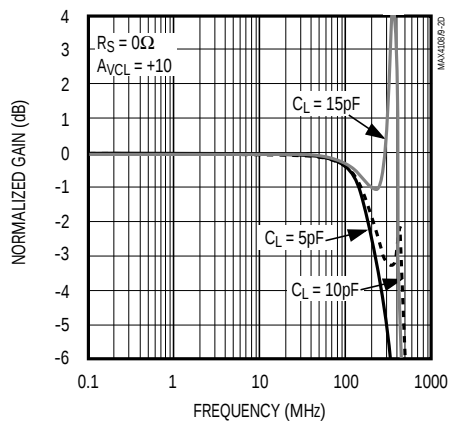
Figure 2d. MAX4309 Response vs. Capacitive Load—No Resistive ( R_S ) Isolation (circuit shown in Figure 1a)
